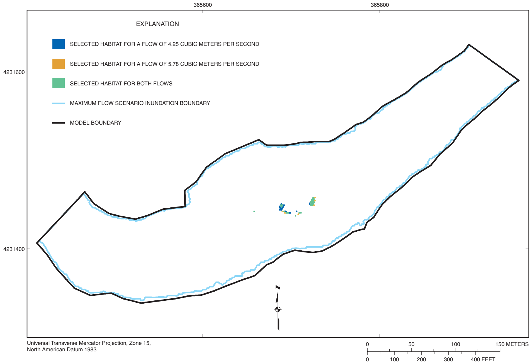
Figure 4-70. Selected habitat area distribution for habitat category 19 (stonecat) at flows of 4.25 and 5.78 cubic meters per second at Marais des Cygnes River site MDC2.
